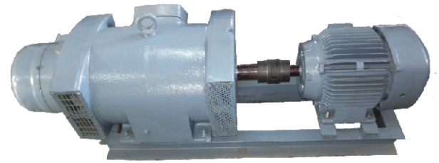
Motor Generator Assembled Unit
